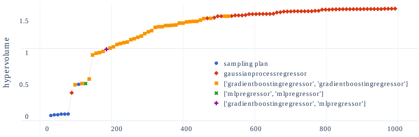
(a) DTLZ4: sampling plan to the 210 configuration
